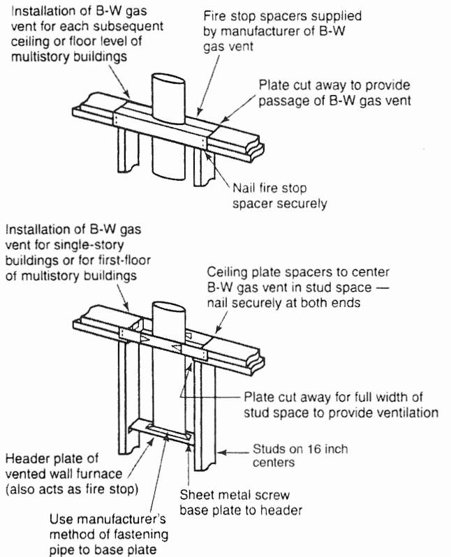
FIGURE 907.1 INSTALLATION OF TYPE B-W GAS VENTS FOR VENTED WALL FURNACES [NFPA 54: FIGURE 10.27.1.3]
