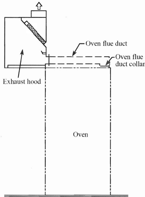
FIGURE 508.8 TYPICAL SECTION OF EYEBROW-TYPE HOOD [NFPA 96: FIGURE 5.1.8.1]
