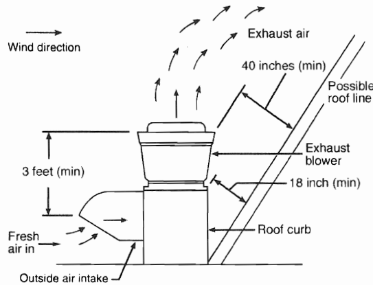
FIGURE 510.9.1 UPBLAST FAN CLEARANCES [NFPA 96: FIGURE 7.8.2.1]
