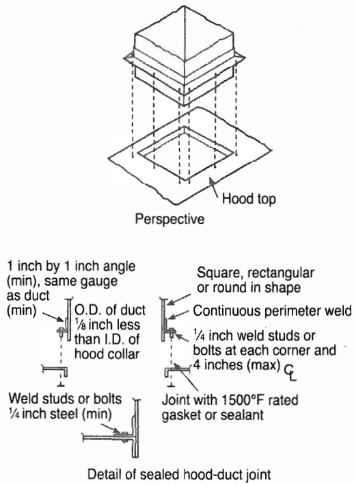
FIGURE 510.5.3 PERMITTED DUCT-TO HOOD COLLAR CONNECTION [NFPA 96: FIGURE 7.5.2.2]
