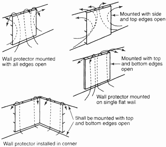
FIGURE 303.10.1(1) 1,2,3 EXTENT OF PROTECTION NECESSARY TO REDUCE CLEARANCES FROM GAS APPLIANCES OR VENT CONNECTORS [NFPA 54: FIGURE 10.3.2.3(a)]
